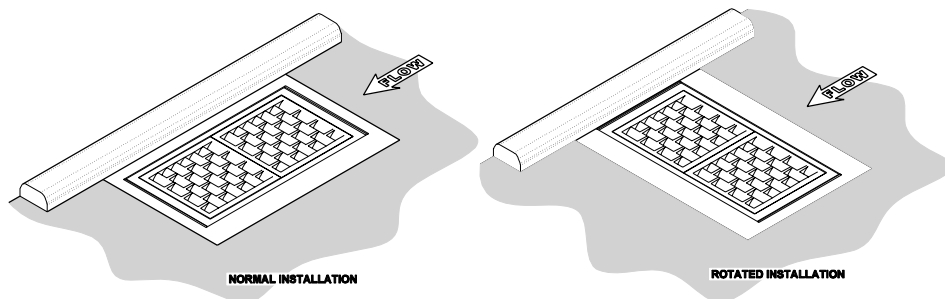
Frame and Vaned Grates For Installation on Grate Inlet
