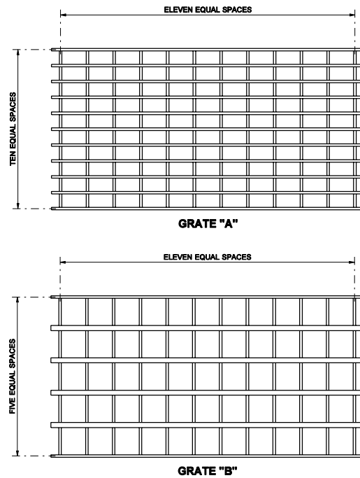
Grate A and B
