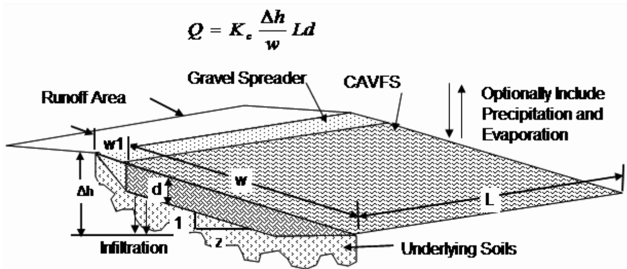
Figure 4-19 CAVFS Detail.
