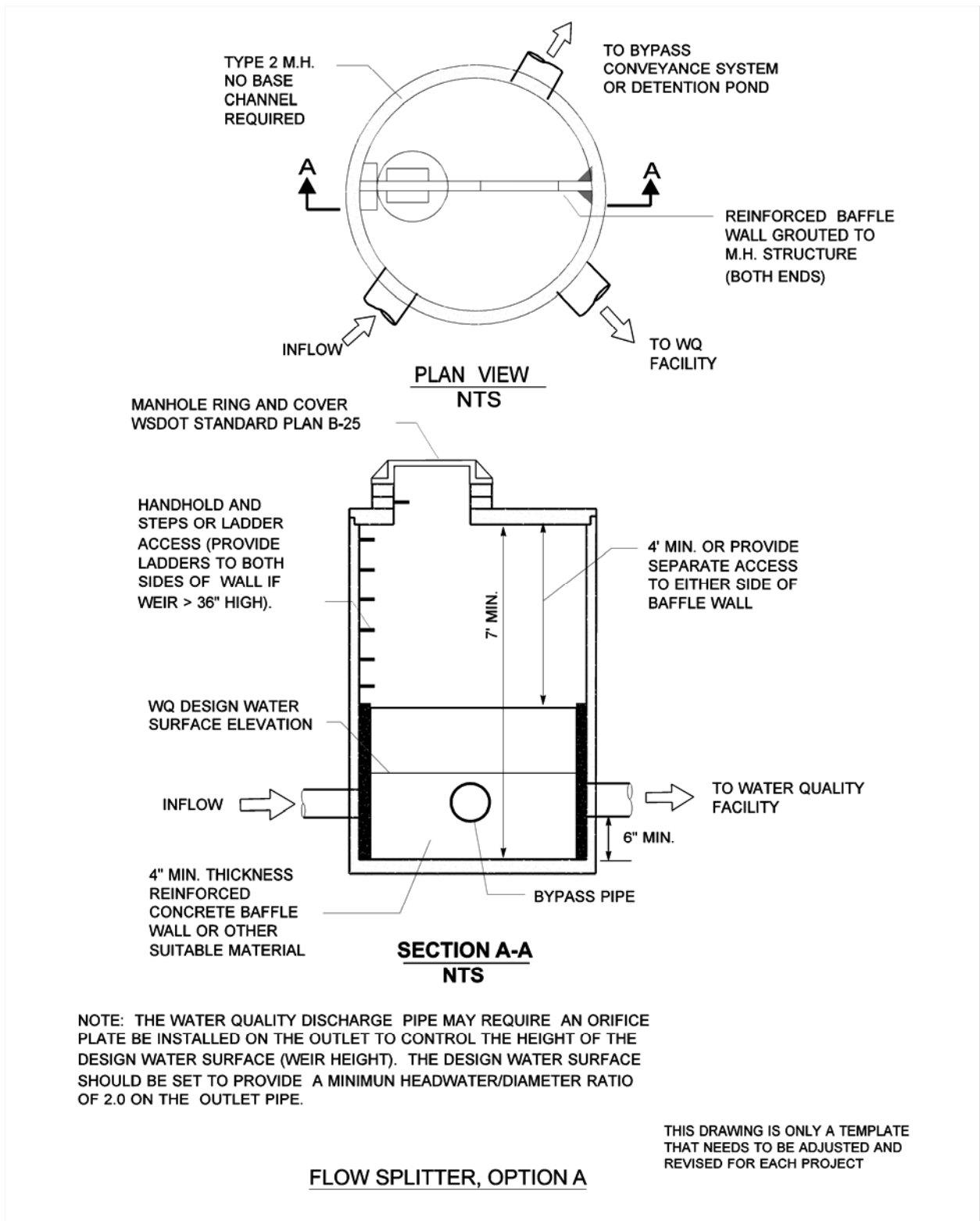
Figure 5.4.3.2. Flow splitter: Option A.
