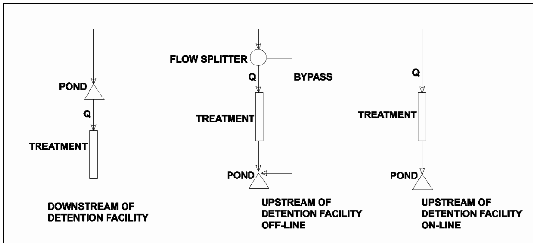
Figure 4-6. Typical on-line and off-line facility configurations.
